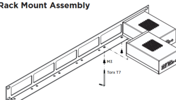
Rack Mount Assembly
